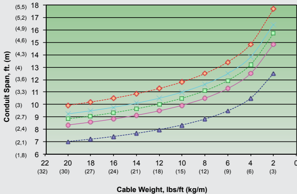
3 ½" (91 mm) SW Conduit (ID only)
