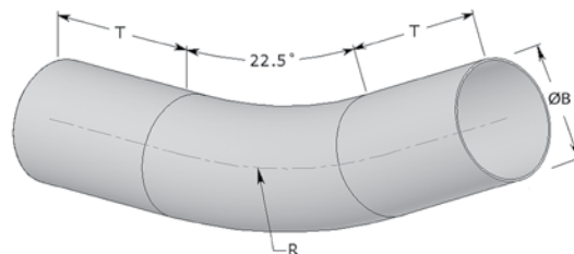
IPS HW 22.5° Elbow
