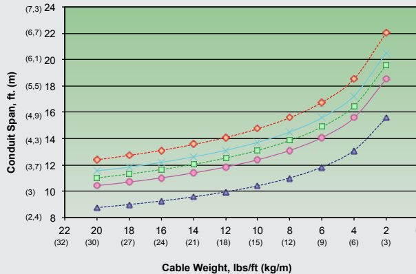
4 ½" (116 mm) SW Conduit (ID only)
